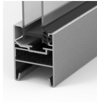
FVE WITHOUT THERMAL BREAK
